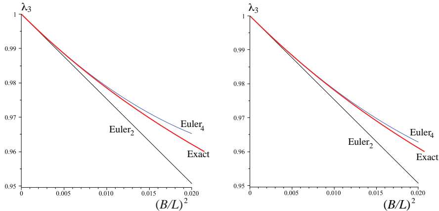
Fig. 1 Comparison of the different Euler formulas obtained by expanding the exact solution to order 2 (classical Euler buckling formula, plot labeled “Euler 2 ”) and to order 4 (plot labeled “Euler 4 ”), for pyrex (figure on the left) and for silica (figure on the right).
