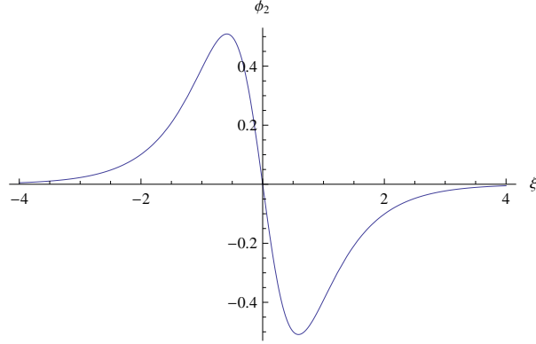
Figure 4: Numeric solution for the second order correction (79) in terms of the angle. ( \xi_0 = 0 , \ell = 10 , E_1 = 1 , E_2 = \frac{1}{2} , \rho_1 = 0.8 , \rho_2 = 1 , \alpha = 0.2 , T = 1 , and the wave speed c is given by (37))
