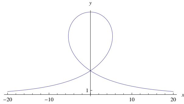
Figure 5: Loop-like traveling wave solution for the homogenous rod, corresponding to the solution (39) for the angle. ( \xi_0 = 0 , \ell = 10 )
