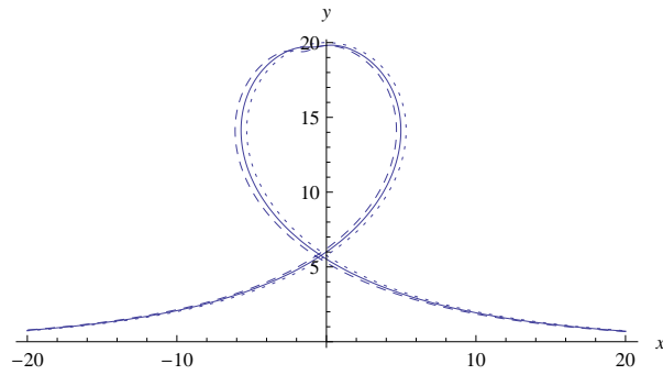
Figure 9: Homogenized solution up to the second correction, \phi = \phi_0 + \epsilon\phi_1 + \epsilon^2\phi_2 , shown in the Cartesian plane for two different values of \epsilon : \epsilon = \frac{3}{8} (solid curve), and \epsilon = \frac{3}{4} (dashed curve). The homogeneous solution ( \epsilon = 0 ) is shown in dotted. ( \xi_0 = 0 , \ell = 10 , E_1 = 1 , E_2 = \frac{1}{2} , \rho_1 = 0.8 , \rho_2 = 1 , \alpha = 0.2 , T = 1 , and the wave speed c is given by (37))
