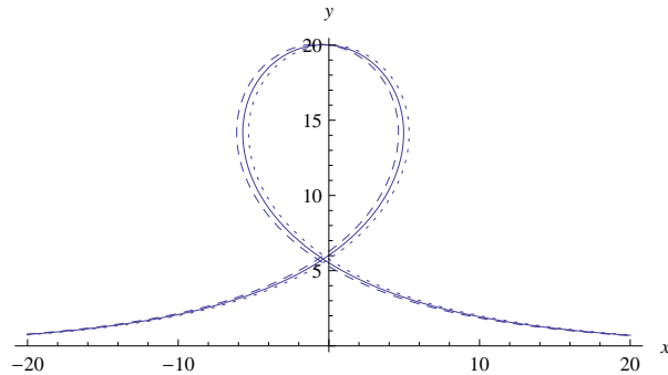
Figure 7: Homogenized solution up to the first correction, \phi = \phi_0 + \epsilon\phi_1 , shown in the Cartesian plane for two different values of \epsilon : \epsilon = \frac{3}{8} (solid curve), and \epsilon = \frac{3}{4} (dashed curve). The homogeneous solution ( \epsilon = 0 ) is shown in dotted. ( \xi_0 = 0 , \ell = 10 )
