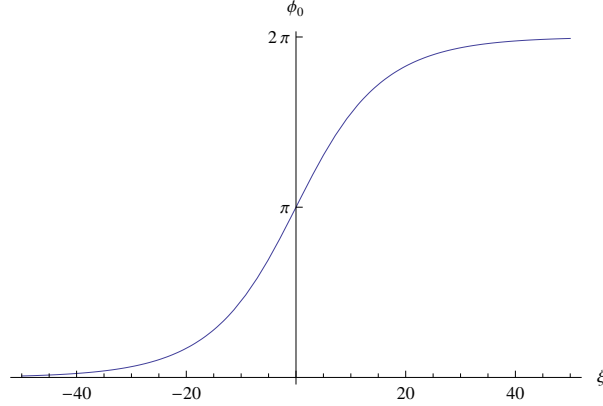
Figure 2: Homogeneous rod solution (39) for the angle. ( \xi_0 = 0 , \ell = 10 )
