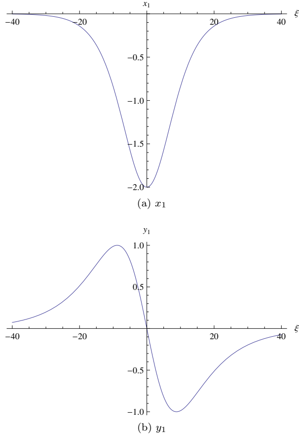
Figure 6: First correction traveling wave solution (83). ( \xi_0 = 0 , \ell = 10 )
