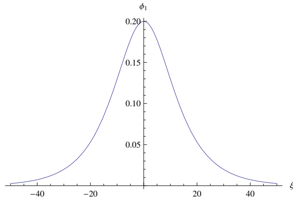
Figure 3: First order correction (57) in terms of the angle. ( \xi_0 = 0 , \ell = 10 )
