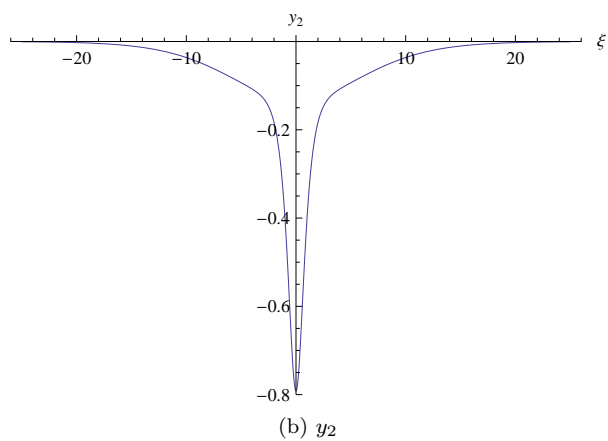
Figure 8: Second correction to the traveling wave solution for the Cartesian coordinates, (84) ( \xi_0 = 0 , \ell = 10 , E_1 = 1 , E_2 = \frac{1}{2} , \rho_1 = 0.8 , \rho_2 = 1 , \alpha = 0.2 , T = 1 , and the wave speed c is given by (37))
